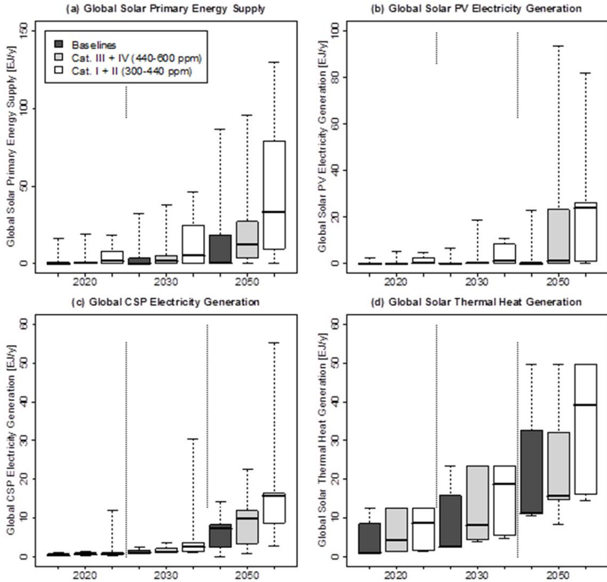
Figure 5: Solar energy across integrated assessment models and scenarios
