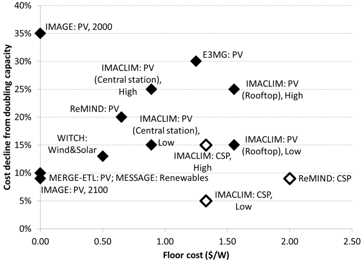
Figure 4: Learning rates and floor costs for models with endogenous technological change in solar electricity generation
