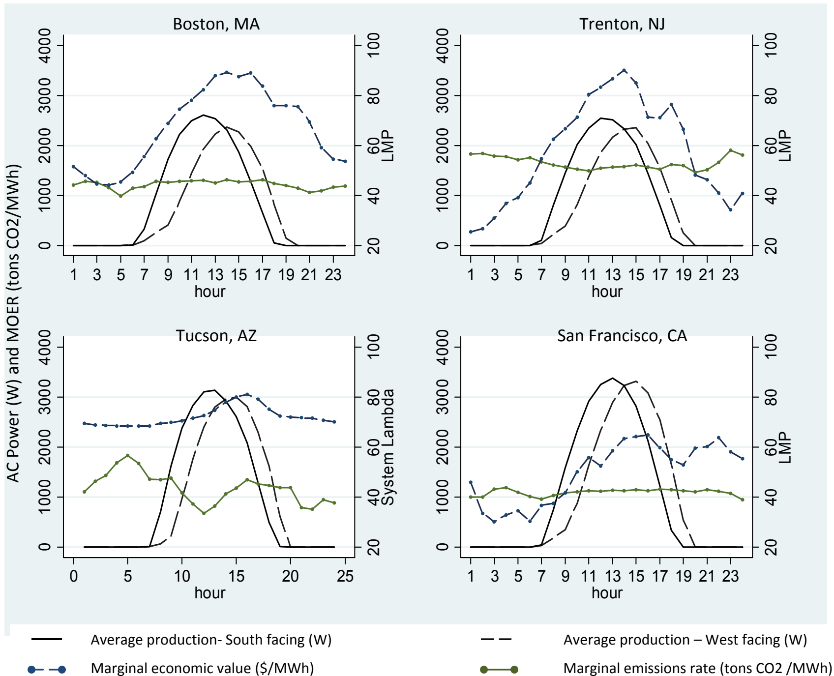
Figure 1 : Daily profiles for simulated electricity generation, emission displacement, and economic value at the four sites
