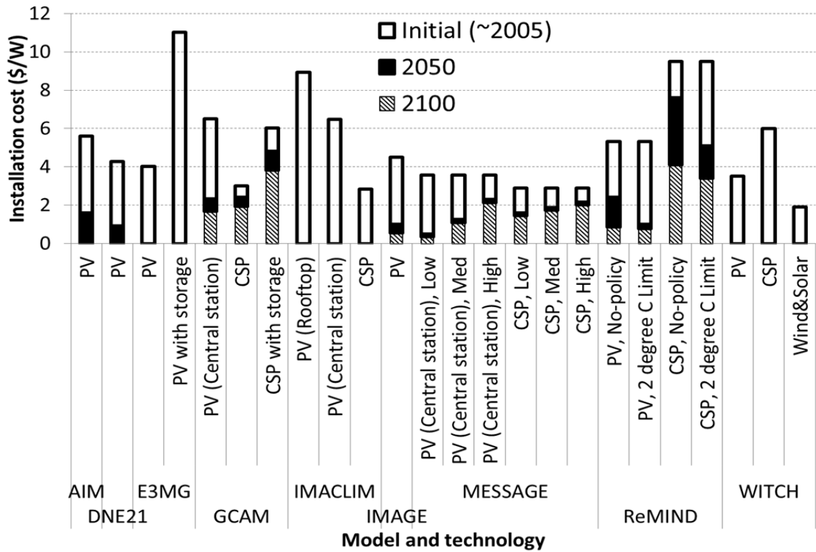
Figure 3: Installation costs by model and solar electricity technology
