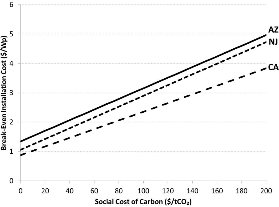
Figure 2: Break-even installation costs corresponding to each social cost of carbon
